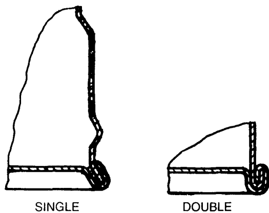
FIG. 3 END SEAMS
