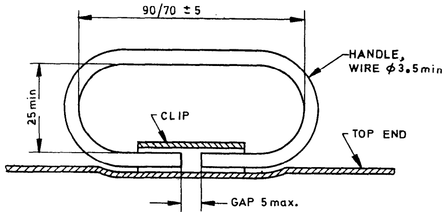
FIG. 6 WIRE HANDLE
