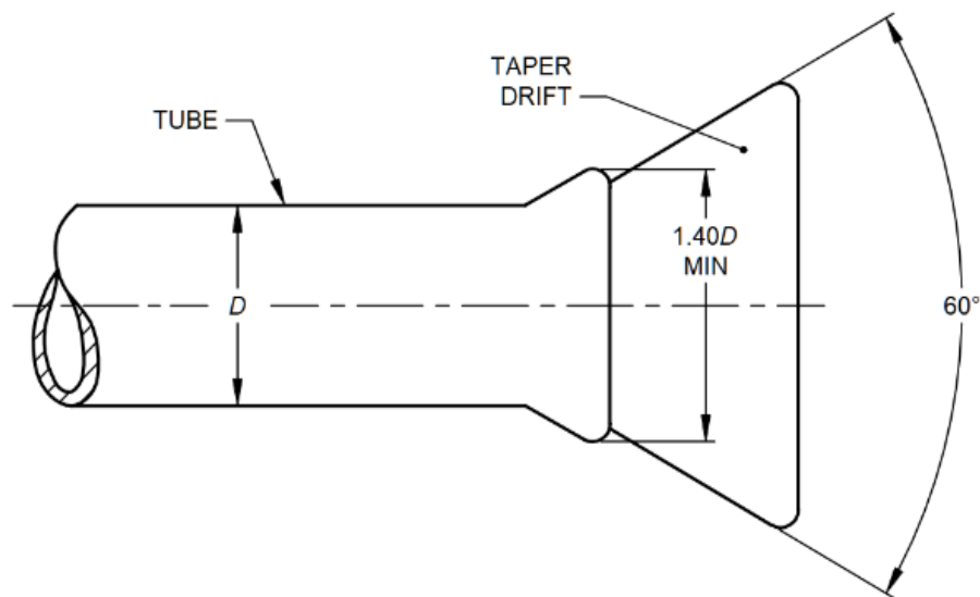
FIG. 2 DRIFT EXPANDING TEST
