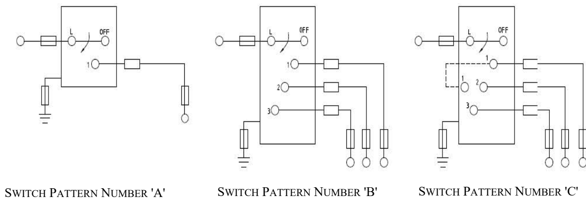
FIG. 1 TYPICAL SWITCH PATTERNS
