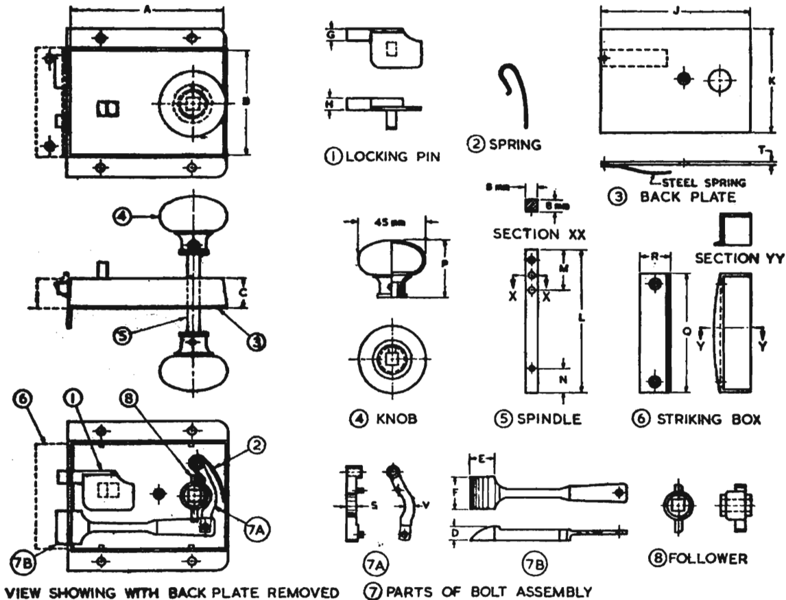
FIG. 1 TYPICAL DESIGN OF RIM LATCH—TYPE 1
