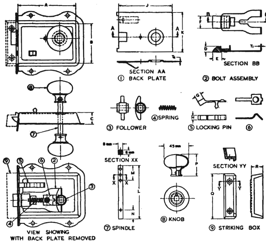
FIG. 2 TYPICAL DESIGN OF RIM LATCH—TYPE 2
