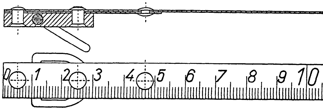
FIG. 4 MEASURE COMMENCING WITH ZERO
